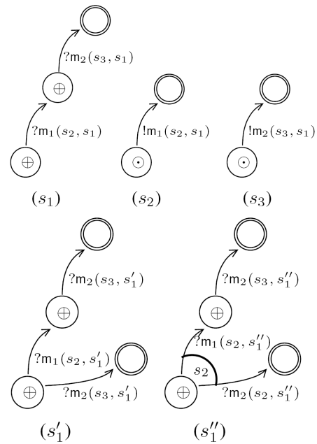
Figure 3: Substituting s_1 by s'_1 causes a race condition, while substituting it with s''_1 does not; the arc in s''_1 expresses the fact that both alternatives are expected from s_2 .
