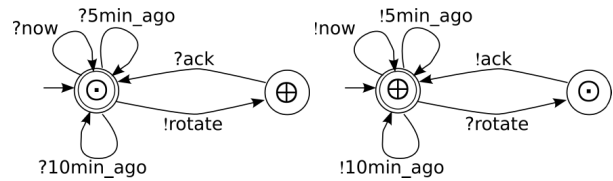
Figure 1: The surveillance interaction protocol: left the Monitor role, right the Sensor role.
